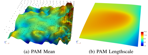
Fig. 3. Prediction and lengthscale maps from the proposed Probabilistic Attentive Mapping (PAM) training paradigm. (a) A higher density of inducing points is allocated to the complex region, enabling the predictive mean to capture finer elevation details. (b) The learned lengthscale map delineates the relatively smooth area on the left (large lengthscale) from the highly varying region near the right boundary (small lengthscale).
