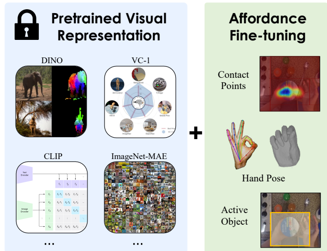
Fig. 1: Pre-trained representations offer a scalable solution to the robotics data bottleneck [63, 69, 56], but existing methods fail to reliably improve over simple baselines like ImageNet [20, 7]. Thus, we present HRP , a method that mines affordances (e.g., contact, hand pose, and object labels) from human videos and uses them to improve self-supervised visual encoders. Our best HRP representation consistently outperforms 6 SOTA baselines by \geq 20\% across 5 diverse tasks and 3 camera views.
