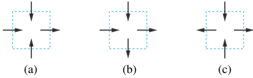
Fig. 18. Three possible flow orientations that cover all possible cases considering flow quantity (which may be zero) and symmetries (flipping of all flow directions and rotating the cell).
