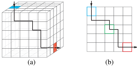
Fig. 21. Illustration of how a certain amount of flow may be routed sideways. Only the top-right-middle 5d_g \times 5d_g \times 5d_g portion of the cell is shown in (a). (b) is a projective view from the front.
