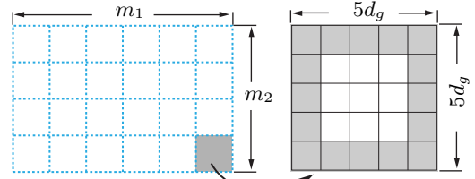
Fig. 10. Partitioning of an m_1 \times m_2 grid into 6 \times 4 cells. Each cell has a size of 5d_g \times 5d_g . Within a cell (the figure on the right), only robots located of a distance no more than d_g from the border may have goals outside the cell.
