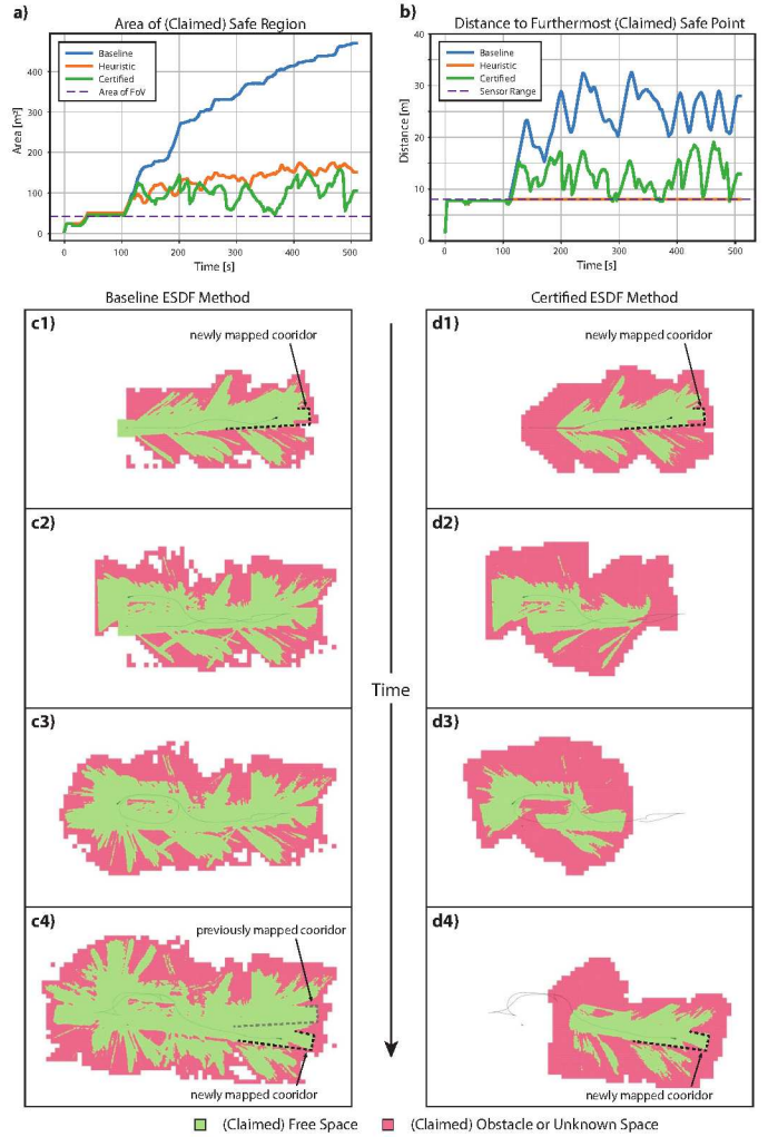
Fig. 8. Quantitative and qualitative analysis of the effect of the deflation on the volume of the certified free space. (a) Compares the area of the claimed safe region on a 2D slice of the ESDF extracted at the robot height. As a reference, the area of the FoV of the camera is also drawn (black dashed line). (b) Compares the distance of the furthestmost (claimed) free voxel from the robot position. As a reference, the maximum depth of the depth sensor (8 m) is indicated (black dashed line). In (c1-c4) we see snapshots of the map generated by the Baseline ESDF method, and in (d1-d4) we see the corresponding snapshots from the Certified ESDF method. The supplementary video animates the map slices.
