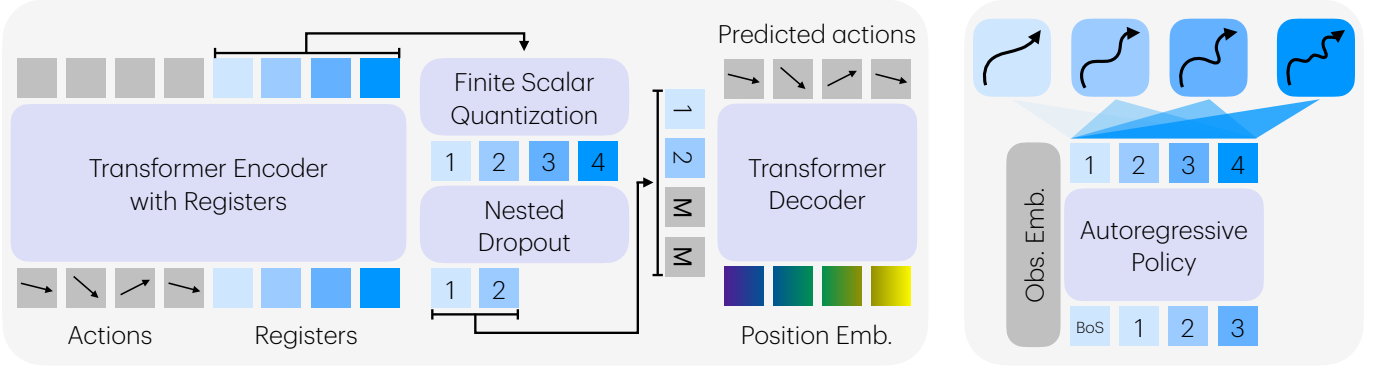
Fig. 3: OAT overview. Left: OAT maps a chunk of continuous actions into an ordered sequence of discrete tokens using a transformer encoder with register tokens, FSQ, and nested dropout to induce token ordering. The resulting tokens form a compact action representation, which is decoded to reconstruct action chunks for downstream autoregressive policies. Right: During OAT policy inference, tokens are generated autoregressively and can be detokenized from any prefix. As more autoregressive steps are taken, additional tokens progressively refine the decoded action chunk, producing actions with increasing temporal and spatial detail. OAT enables flexible, anytime action generation.
