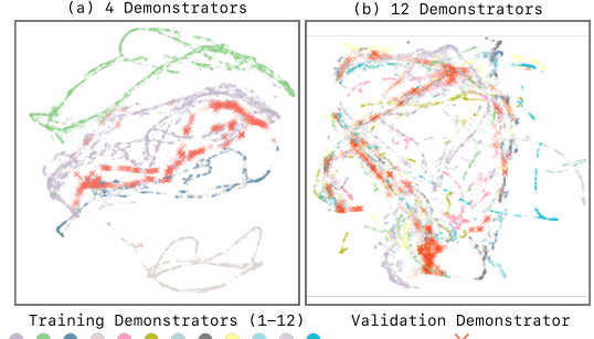
Fig. 12: Demonstrator Diversity Visualization. We visualize UMAP embeddings of encoded features for 4 and 12 demonstrators in the multi-scene demonstrator scaling setting, showing greater overlap between training and validation demonstrators with increased demonstrator diversity.
