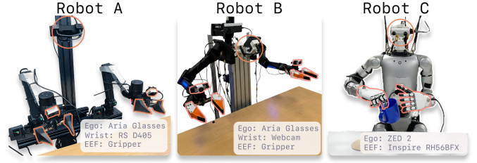
Fig. 6: Robot Platforms. We perform evaluation on three distinctive robot platforms across labs with shared protocols.
