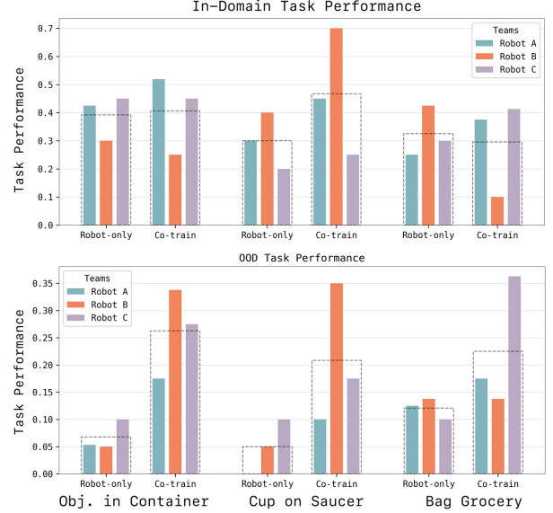
Fig. 9: Co-training improves transfer. Joint training with human egocentric data consistently improves in-domain performance and out-of-domain generalization across robots.
